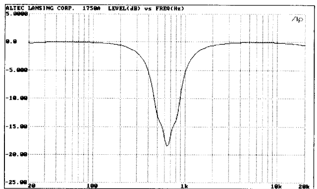
630 Hz Filter Set at -15 dB, 500 Hz and 800 Hz Filters Set at -6 dB
