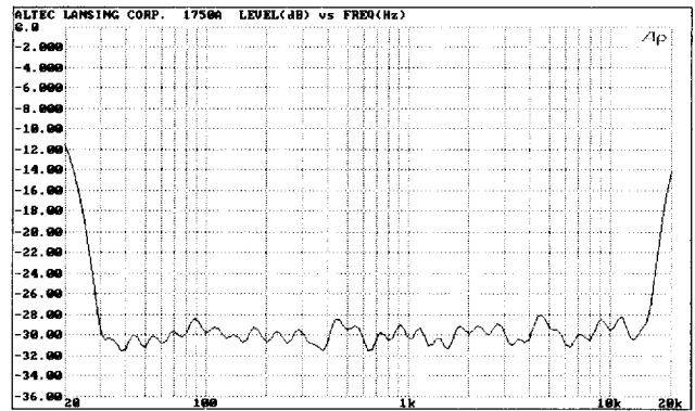
All Filters Set at Full Attenuation
