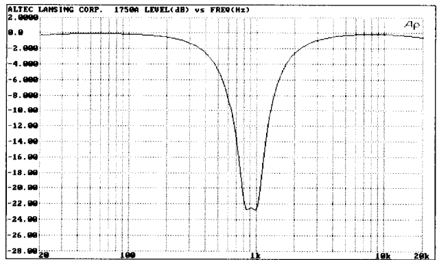
Two Adjacent Filters, 800 Hz and 1 kHz, Set at Full Attenuation
