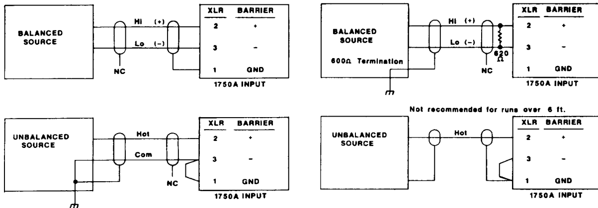
Figure 3. Typical Input Connections
