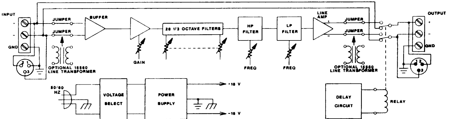
Figure 7. Block Diagram of the 1750A
