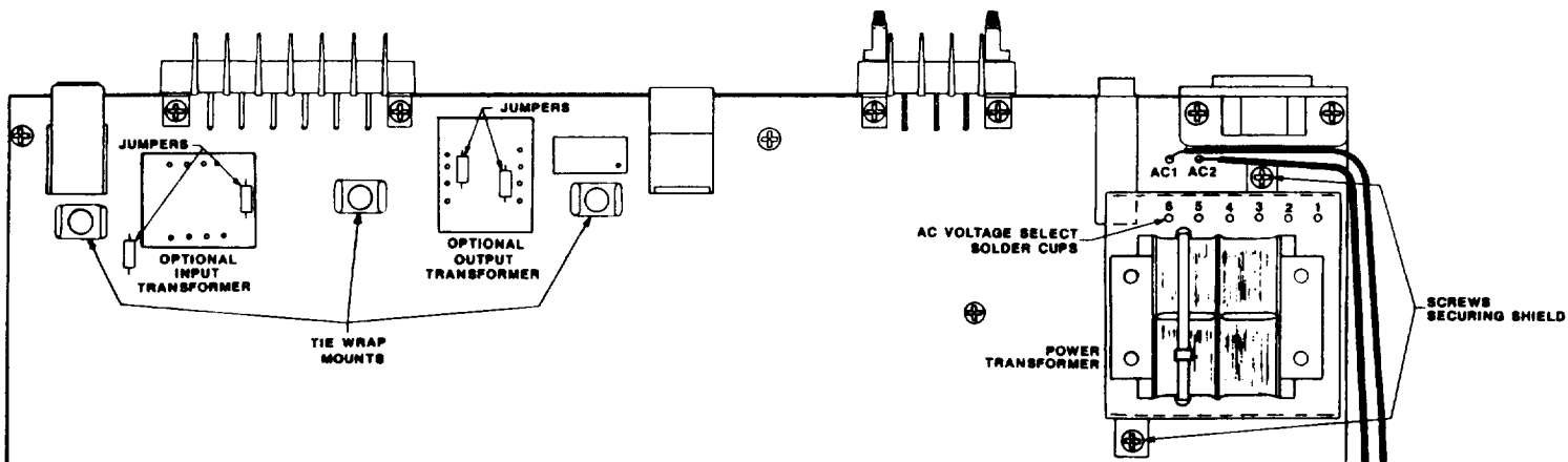
Figure 1. Location of Pertinent Components on Circuit Board.
