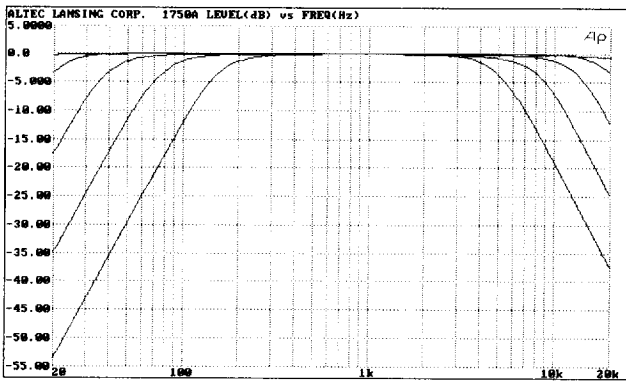
High-Pass and Low-Pass Functions (18 dB/oct) Independently Plotted
