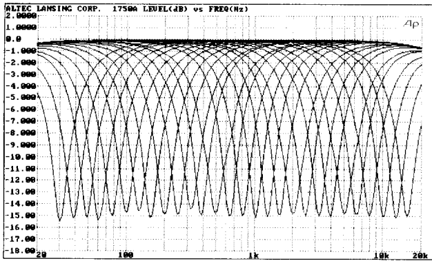
28 \frac{1}{3} Octave Filters at Maximum Attenuation (-15 dB). Each Independently Plotted
